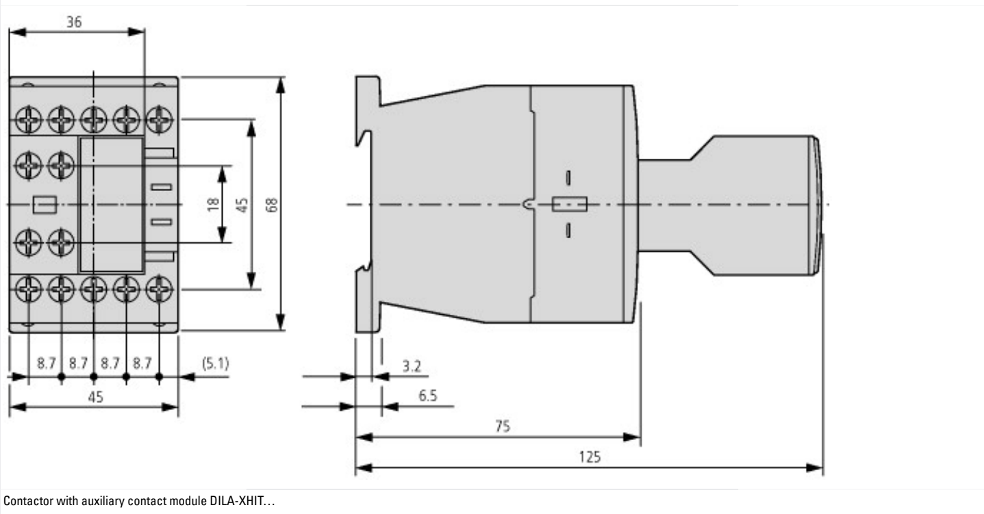
Contactor with auxiliary contact module DILM32-XHI.../DILA-XHI...
