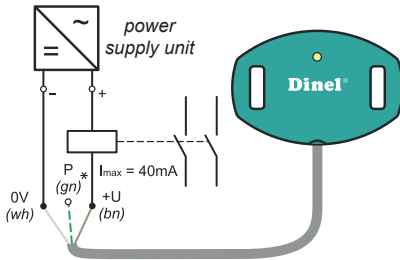
Connecting of the sensor FLD-32 to the relay coil
