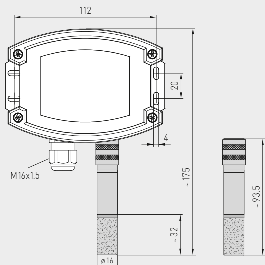
Dimensional drawing
