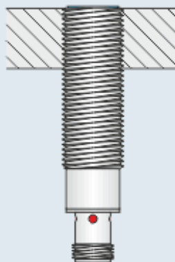
Flush mounting
