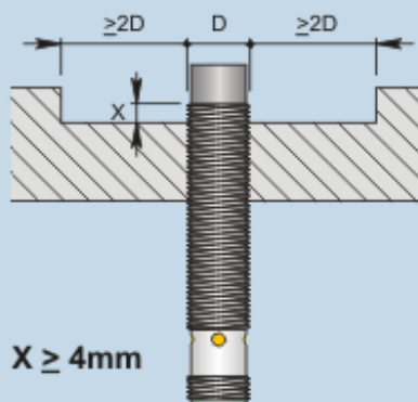
Non flush mounting
