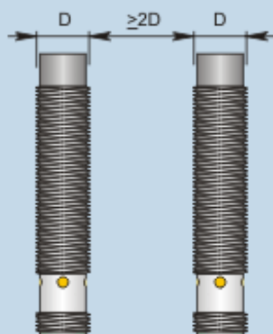
Side by side mounting
