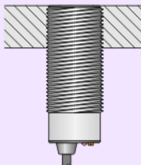
Flush mounting
