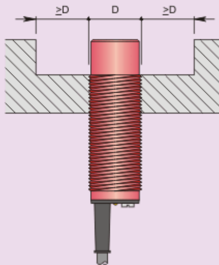
Non flush mounting
