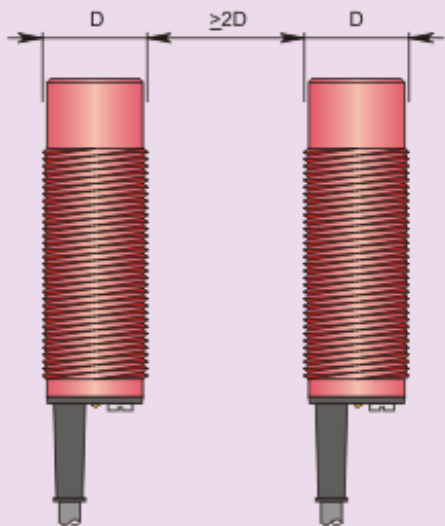
Side by side mounting
