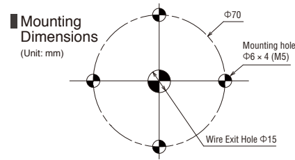
Wall Mount Bracket (For \Phi 150\text{mm} ) SZK-103
