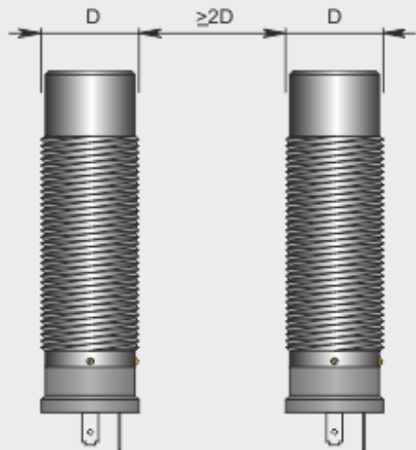
Side by side mounting
