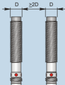
Side by side mounting
