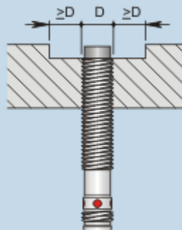
Non flush mounting
