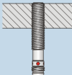
Flush mounting
