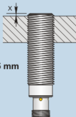
Flush mounting
