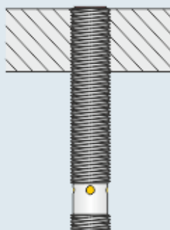
Flush mounting
