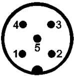
S85-Y03-00V Voltage version
