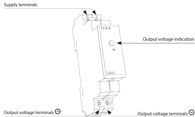
PS-10-12
