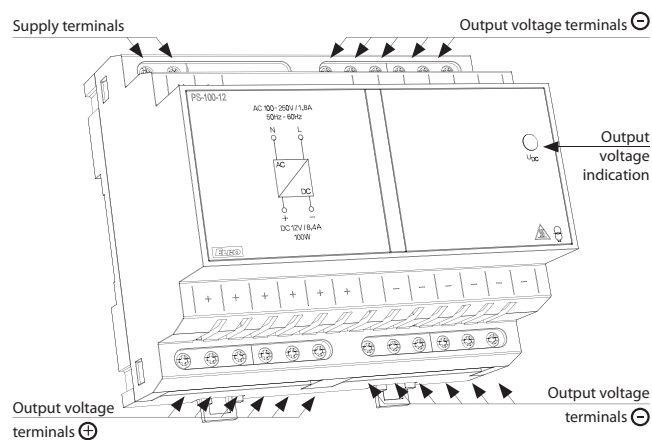
PS-100-12
